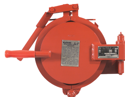
■ 8-inch D2000 Clamp Ring Closure
