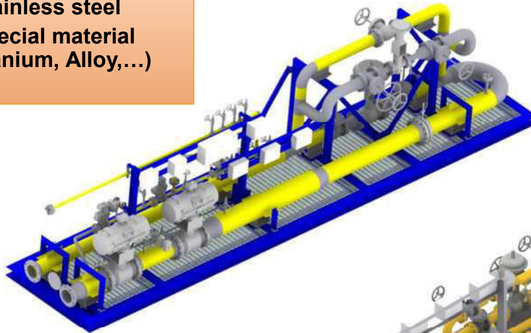
Feeding Fuel Skid for Vacuum Degassing Unit
